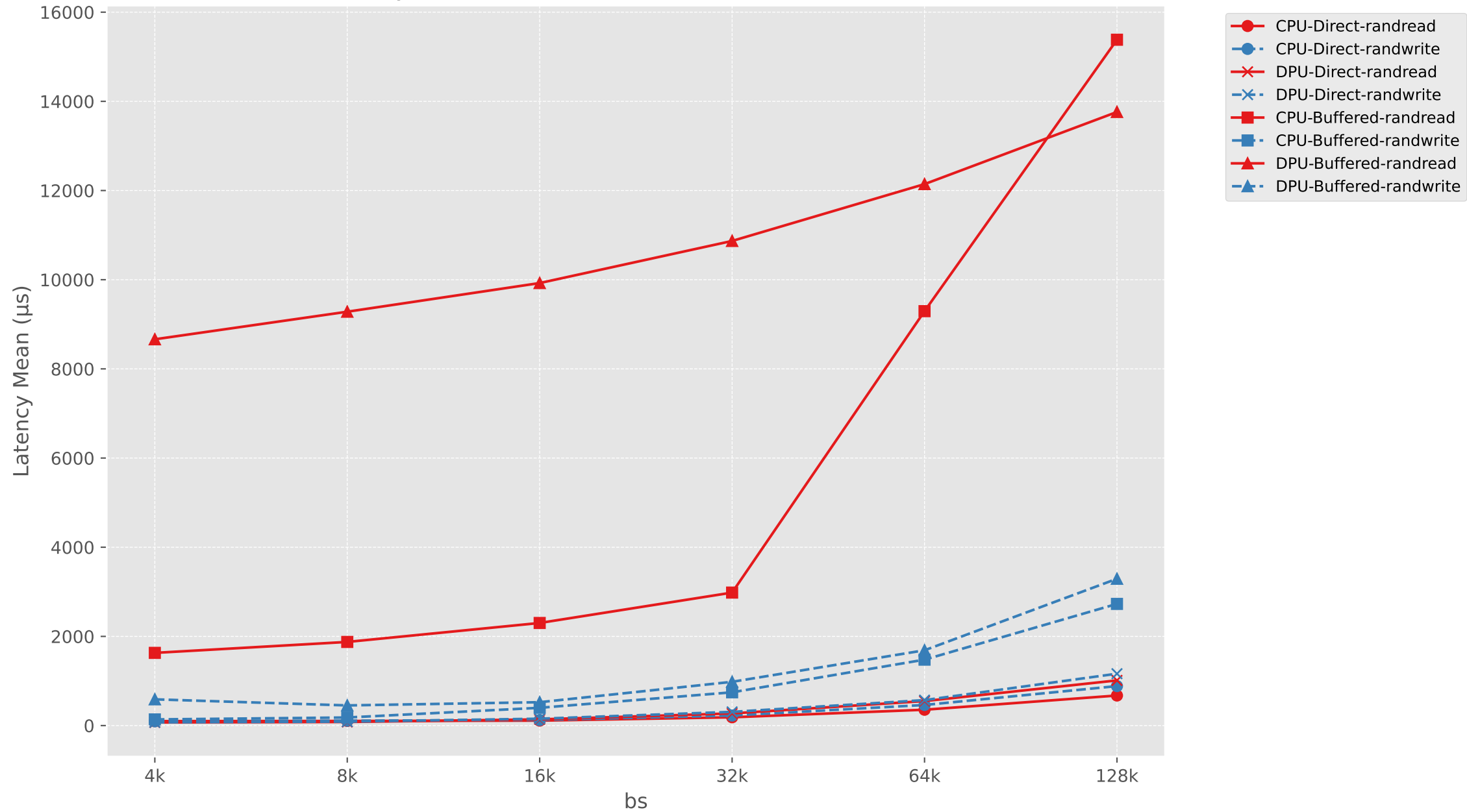
Latency Mean vs bs (CPU vs DPU, Direct vs Buffered)
